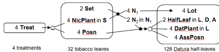
Figure 17: Factor-allocation diagram for McIntyre's (1955) two-phase experiment: treatments are randomized to tobacco leaves and tobacco leaves are randomized to Datura half-leaves; the arrow to the \ominus , the \oplus and the two lines from the \oplus indicate that Treat is randomized to the combinations of NicPlant and Posn using an orthogonal design; N_1 is a pseudofactor indexing the pairs of tobacco plants formed by taking a plant from each set in the first phase and N_2 is a pseudofactor indexing the tobacco plants within the pairs formed by taking a plant from each set in the first phase; N_1 is randomized to Lot in the second phase; the combinations of N_2 and Posn is randomized to the combinations of HalfLeaf, DatPlant and AssPosn using a nonorthogonal design, the latter indicated by the \circ ; S = Set; L = Lot; D = DatPlant; A = AssPosn.
